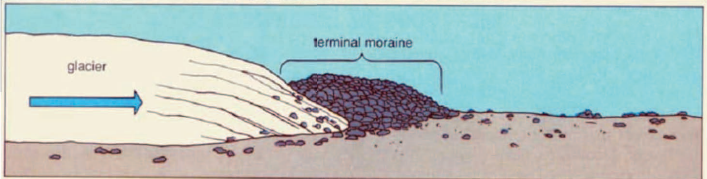
16B-3 A terminal moraine is a ridge of rock debris that a glacier piled up at its front.
