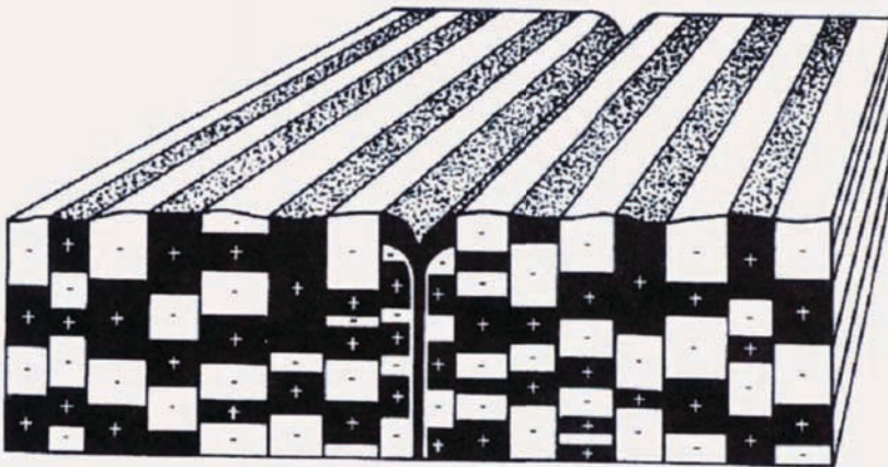
Figure 8: Drilled cores show chaotic paleomagnetic patterns, providing evidence for rapid spreading and rapid reversals along the rift.
