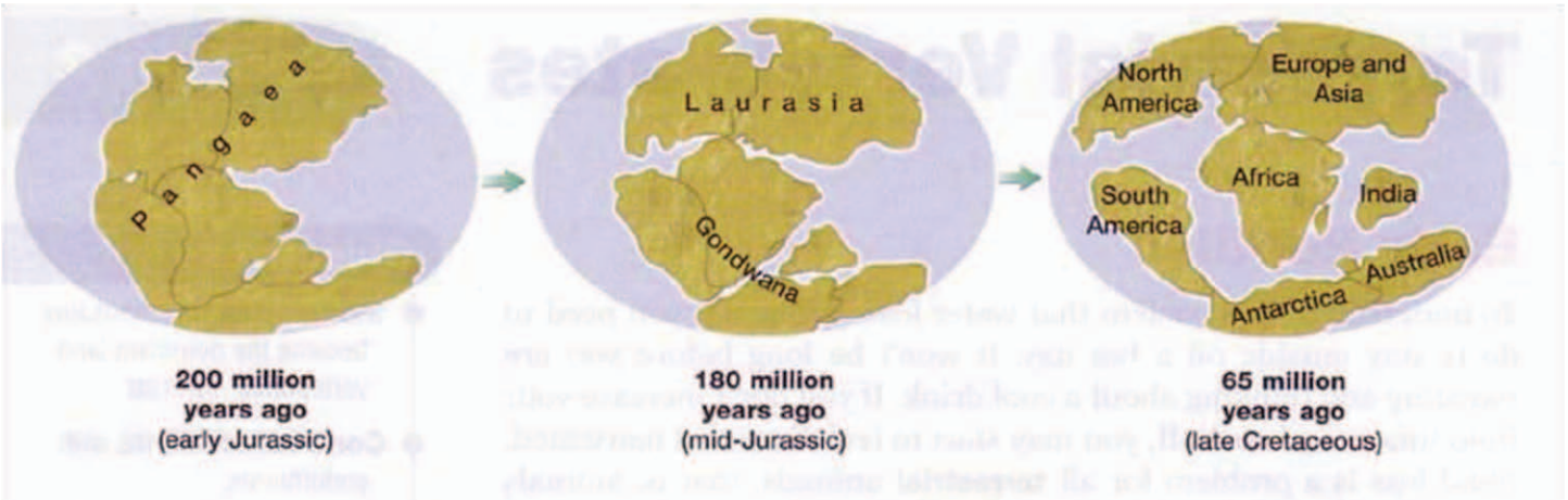
Figure 12 Breakup of Pangaea. The supercontinent Pangaea began to break up during the Jurassic period. By the late Cretaceous period today's continents began to be recognizable.
