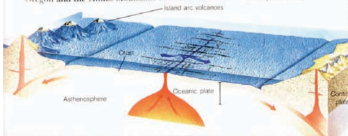
Figure 10-3 Many volcanoes form where plates collide.
